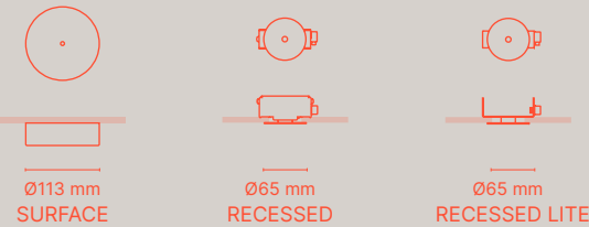
PIASTRA ROTONDA / ROUND PLATE
